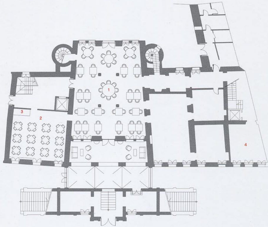
RESTAURANT PLAN
